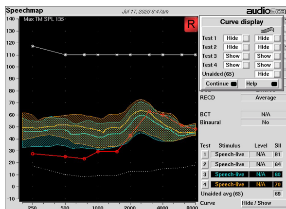
Figure 6. Long-term speech levels measured at the listener’s eardrum for conversational-level speech measured at a talker-listener distance of six feet when an N95 face mask is worn for the Normal program (teal curve) versus when Edge Mode is activated (orange curve).
